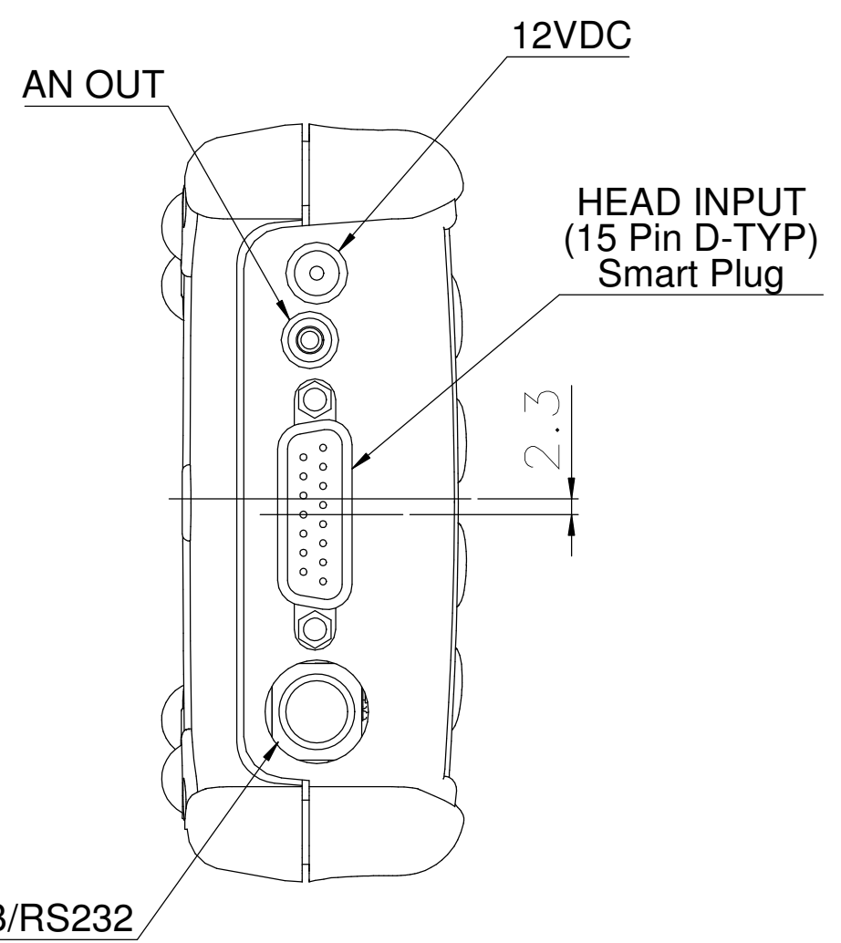
VIEW A
